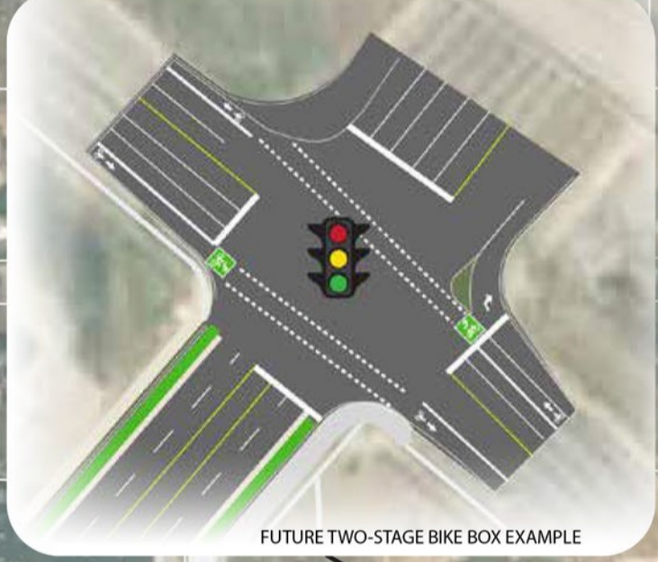
FUTURE TWO-STAGE BIKE BOX EXAMPLE
